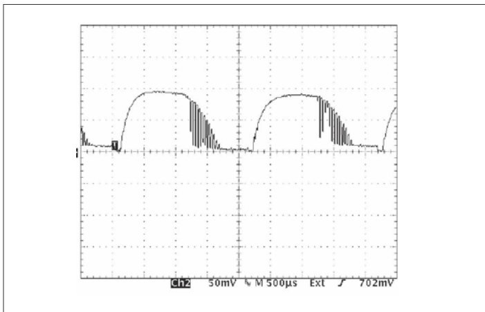
Figure 5: Revised current waveform showing the shaping introduced at the end of the commutation cycle
