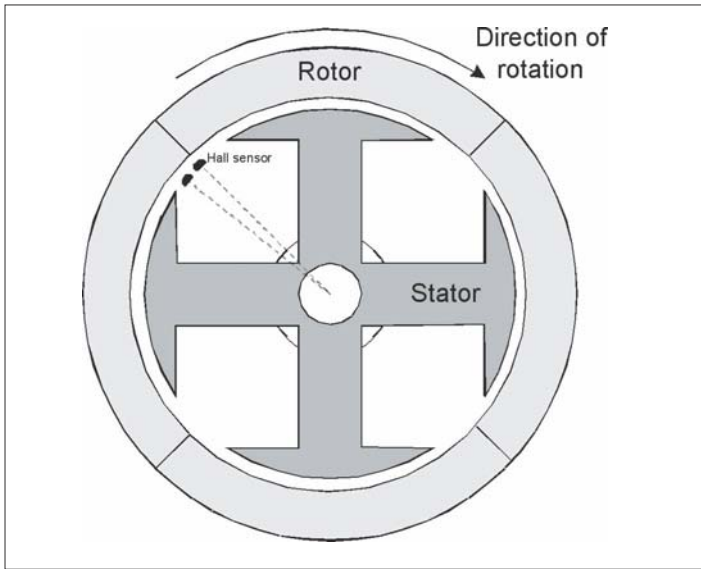
Figure 4: Topography of a 4-pole BLDC motor showing Hall device advance
