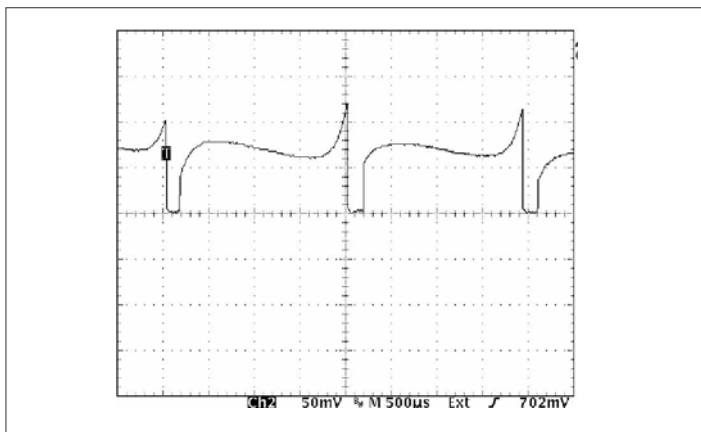
Figure 1: Typical BLDC motor supply current waveform
