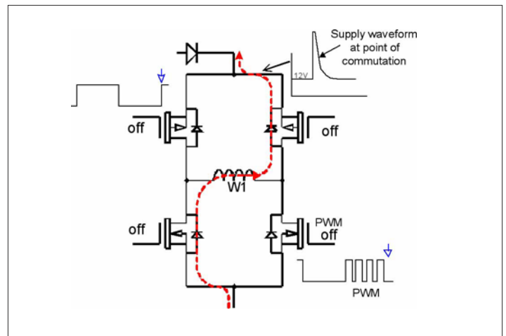
Figure 2: Attempted current path and resultant charge-pumping effect on supply
