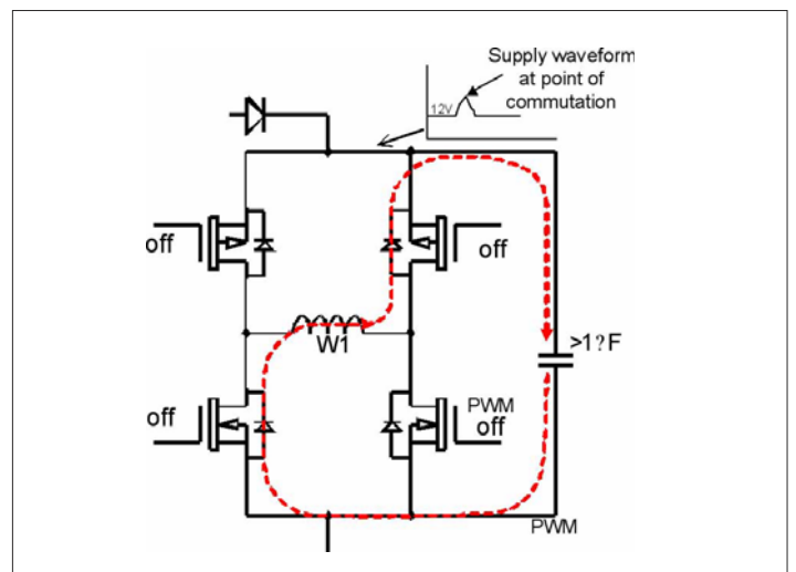
Figure 3: Removing the effects of back emf with a capacitor.
