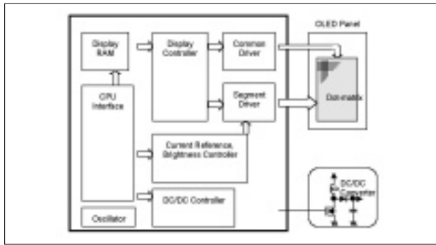
Figure 5: Functional Block Diagram of an Integrated OLED Driver
