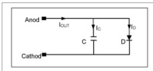
Figure 2: Electrical Model of an OLED Pixel
