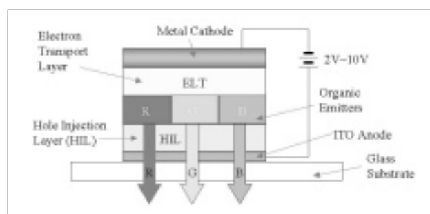
Figure 1: OLED Device Structure
