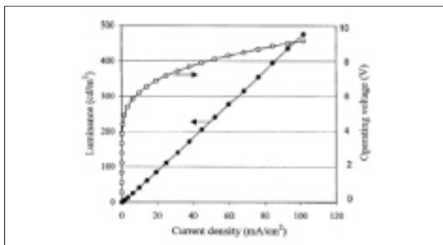
Figure 6: BVI Curve of a Pixel on an OLED panel
