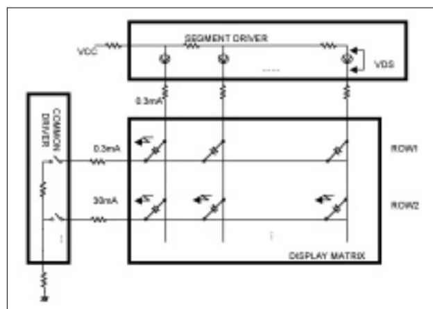
Figure 4: Display Pattern Dependent Variations
