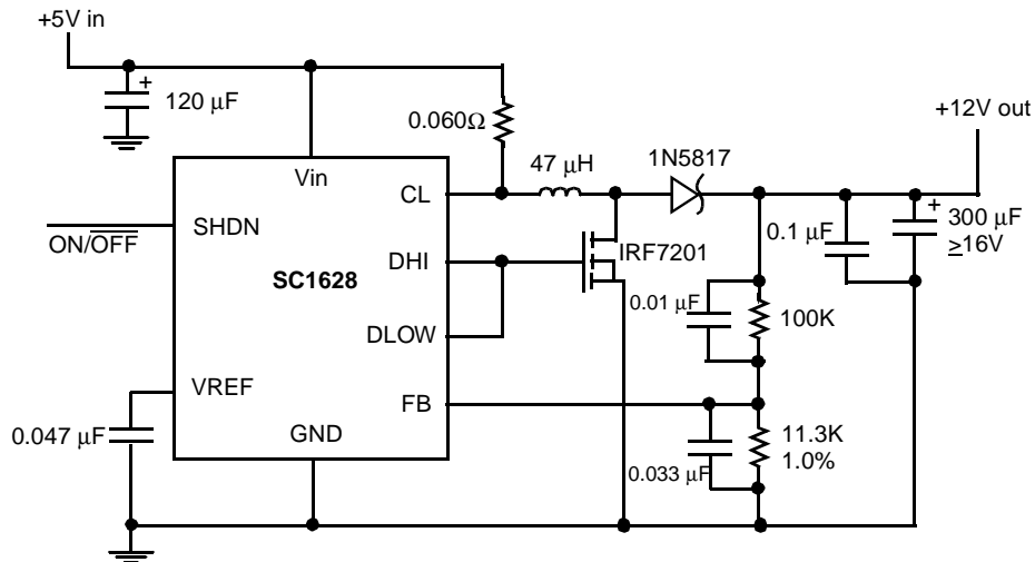
Figure 4. Semtech Schematic
