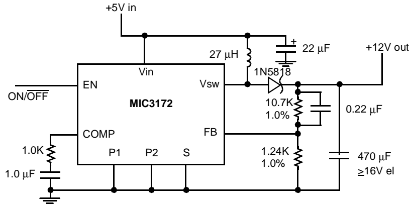
Figure 3. Micrel Schematic
